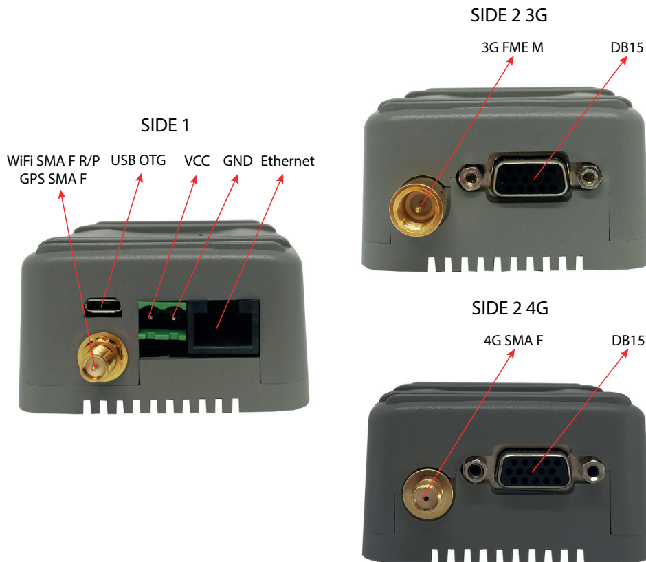
Illustration 2: MTX-GTW external interfaces
