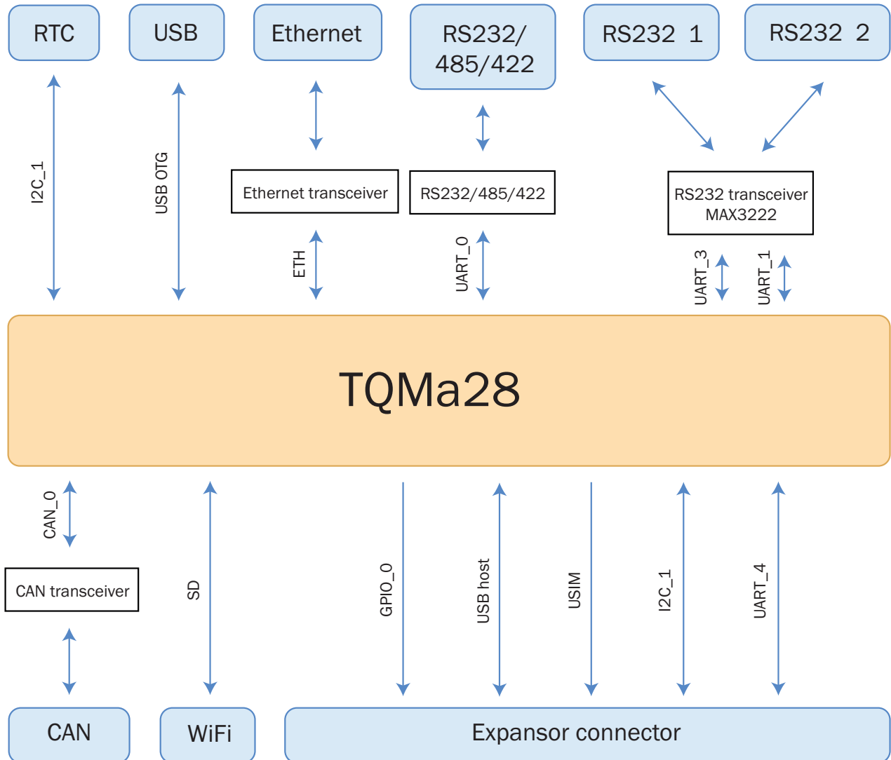
Illustration 1: MTX-GTW block diagram
